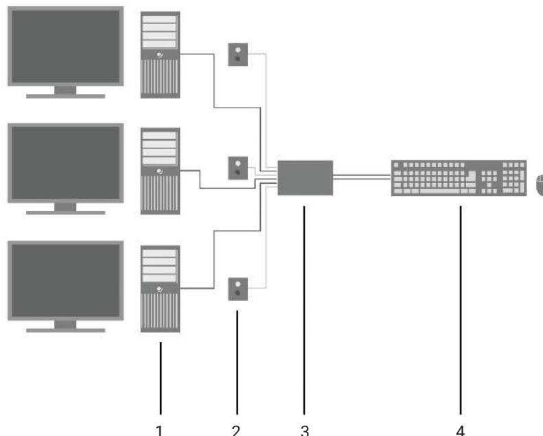
FIGURE 3-1. DIRECT CPU CONNECTION
