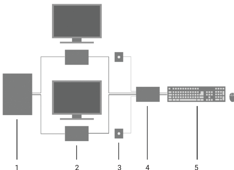
FIGURE 3-2. USING THE TC KM SWITCH WITH A BLACK BOX KVM SWITCH
